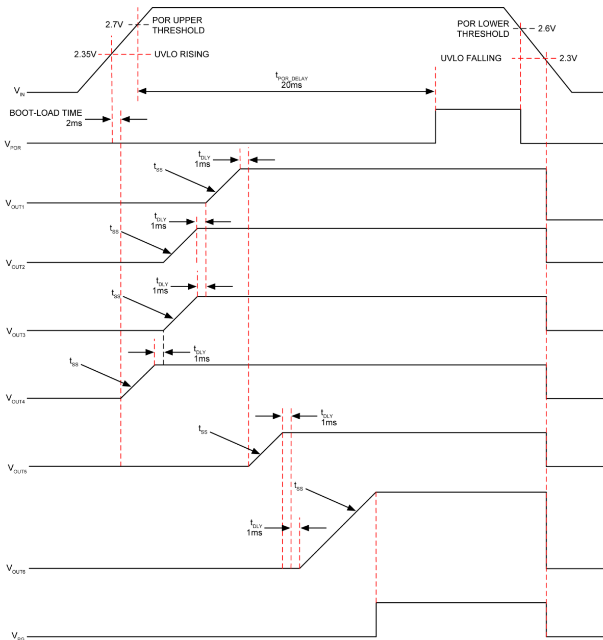
Figure 17. MIC7401 Power-Up/Down
