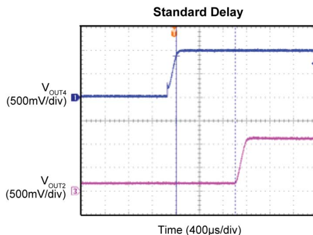
Figure 14. Standard Delay Time
